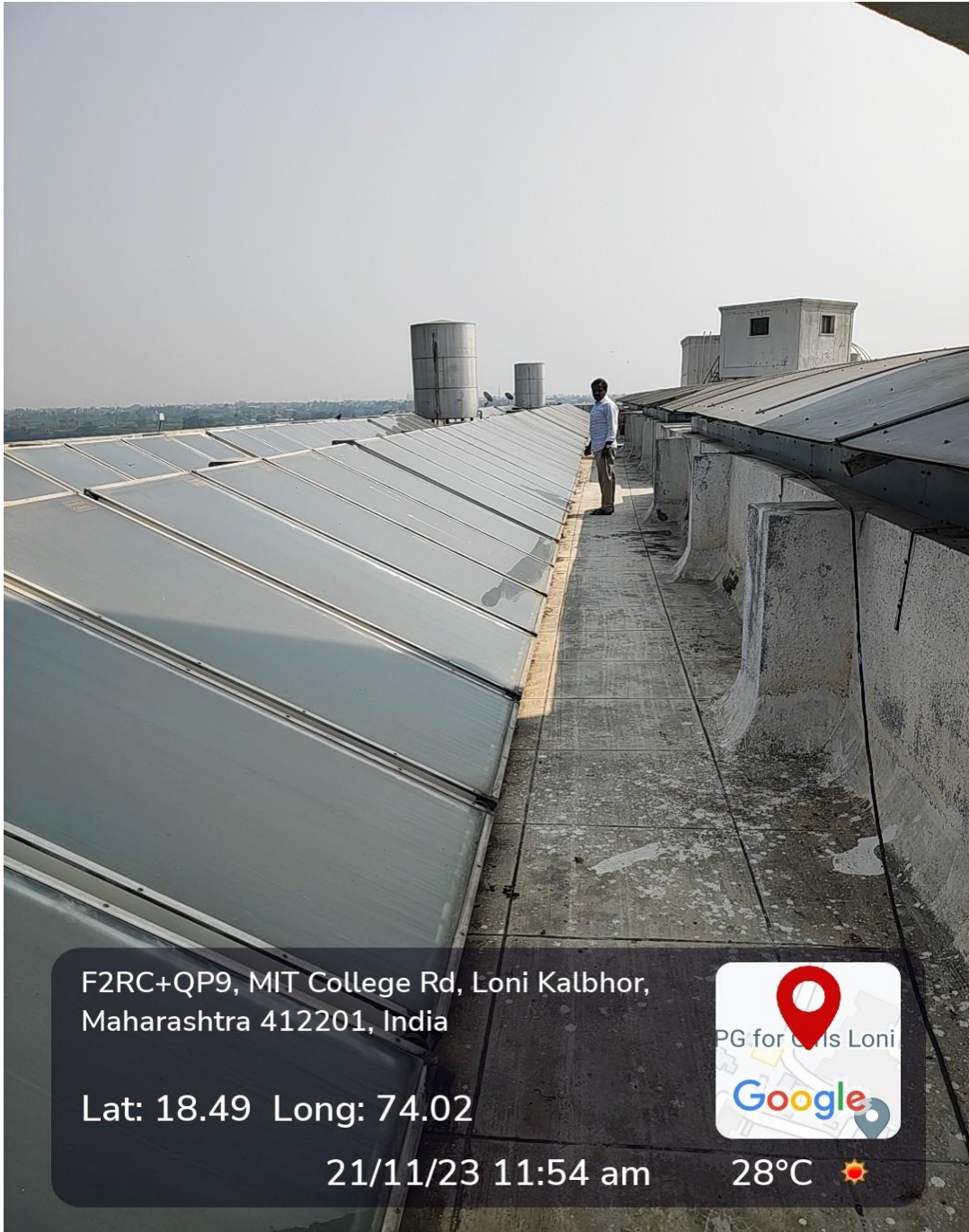
Geotagged Photograph of Solar Panel for Solar Water Heating System
